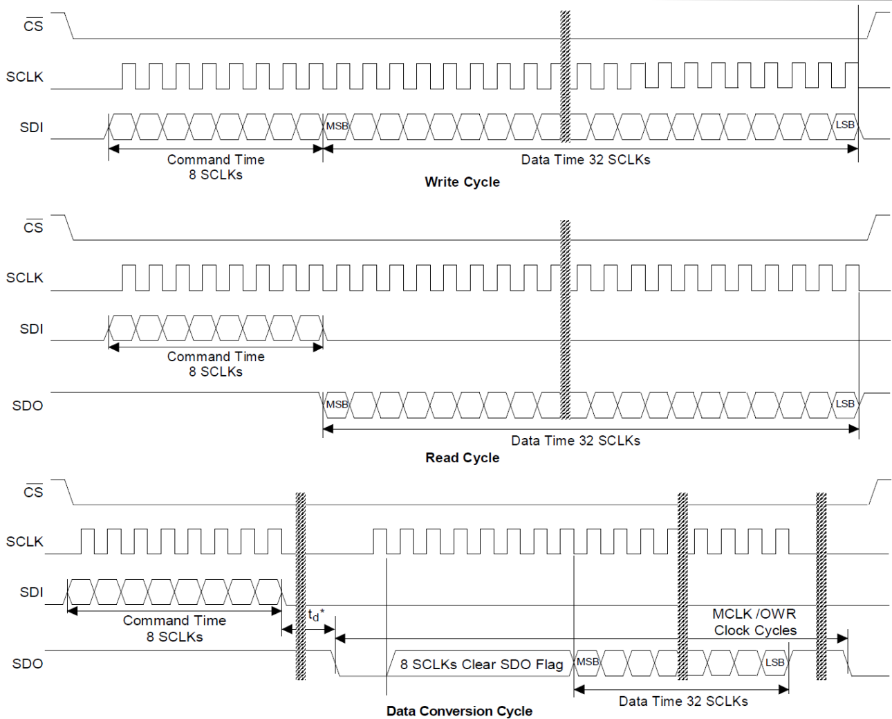
Figure 21. Command and Data Word Timing
