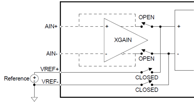
Figure 23. Self Calibration of Gain
