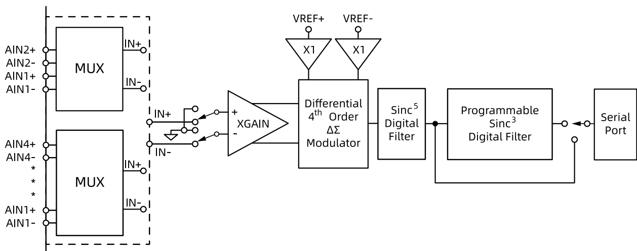
Figure 19. Multiplexer Configuration
