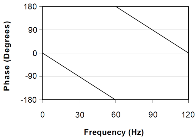
Figure 29. 120 SPS Filter Phase Plot to 120 Hz
