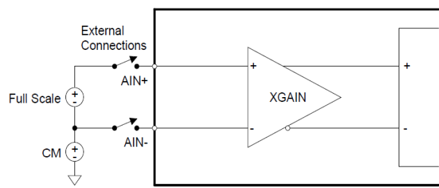
Figure 25. System Calibration of Gain
