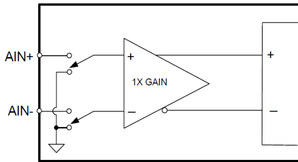
Figure 22. Self Calibration of Offset
