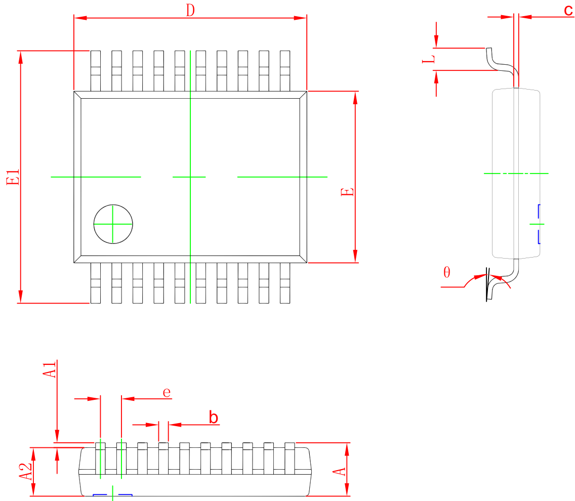
SSOP20(209mil) PACKAGE OUTLINE DIMENSIONS
