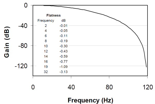
Figure 28. 120 SPS Filter Magnitude Plot to 120 Hz
