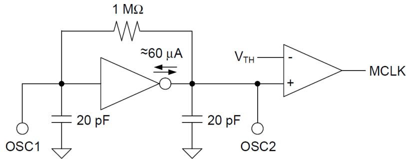
Figure 31. On-chip Oscillator Model
