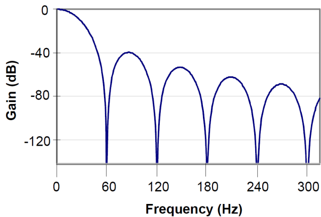
Figure 27. Digital Filter Response (WR = 60 SPS)
