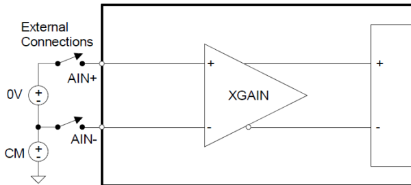
Figure 24. System Calibration of Offset
