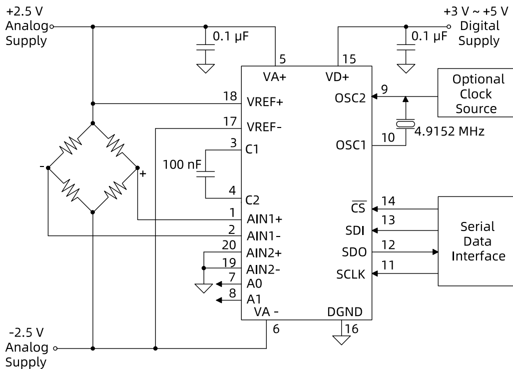
Figure 33. LHA7532B Configured with \pm 2.5 V Analog Supplies
