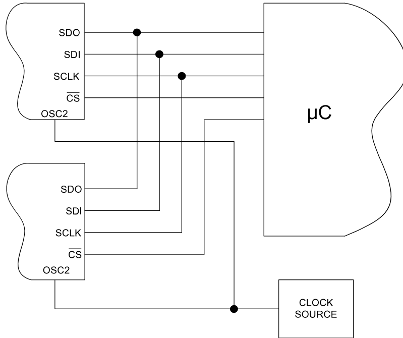
Figure 26. Synchronizing Multiple ADCs
