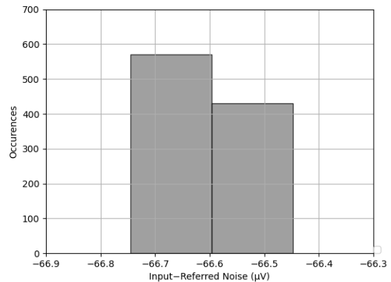
Figure 4. Histogram (Output Data Rate = 5 SPS, PGA gain =1)
