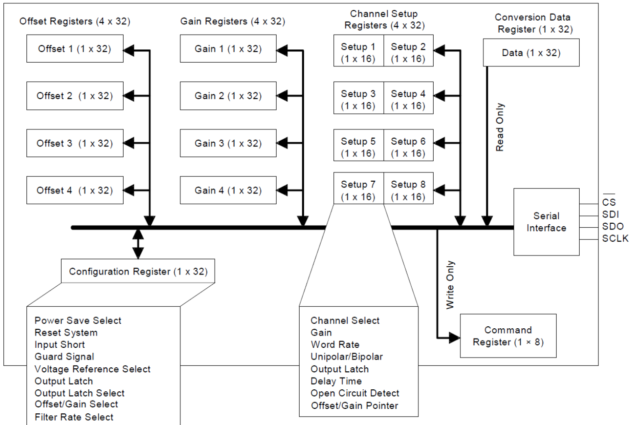
Figure 20. LHA7532B Register Diagram
