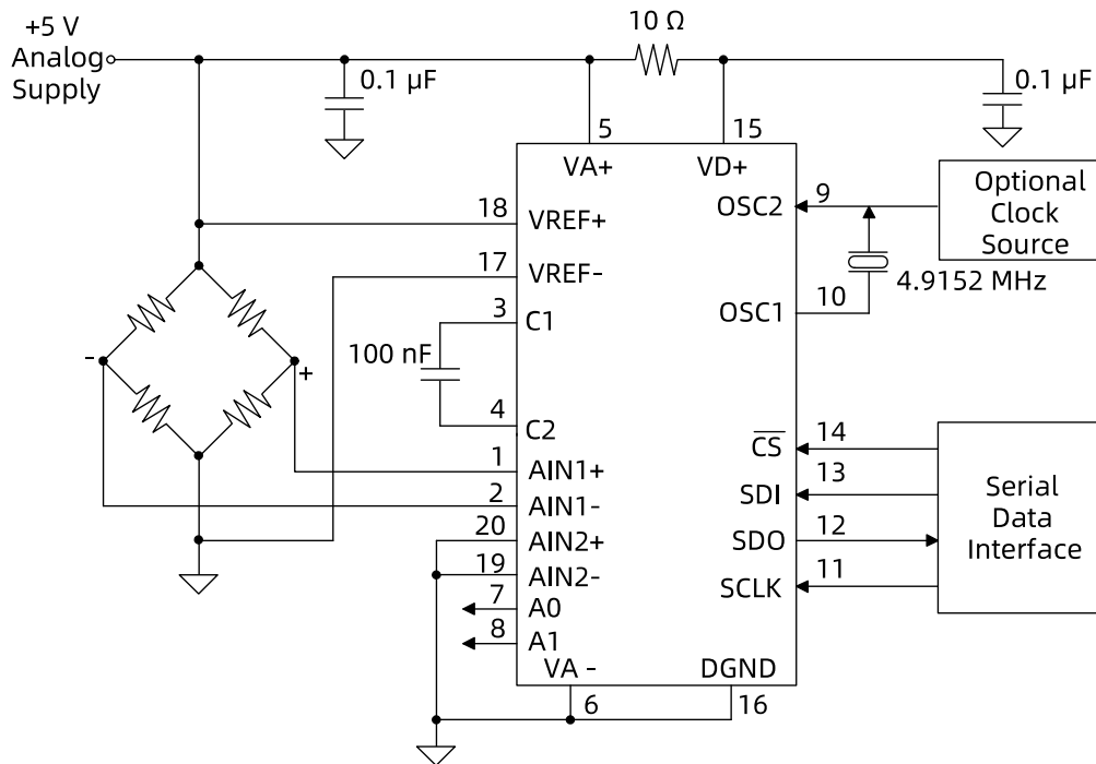
Figure 32. LHA7532B Configured with a Single +5 V Supply
