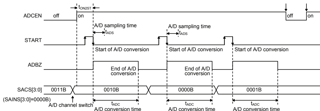
A/D Conversion Timing
