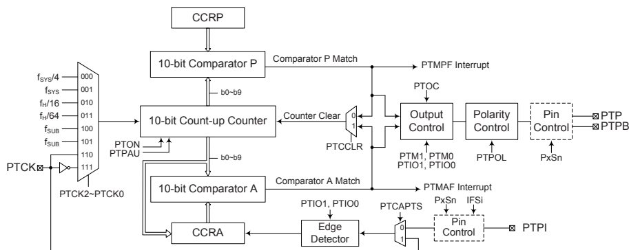
Periodic TM Operation
