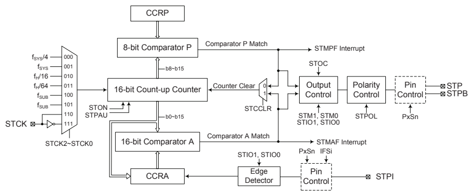
Standard Type TM Block Diagram
