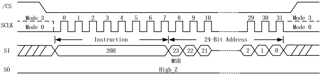
Figure 7.4.5. Sector Erase Instruction
