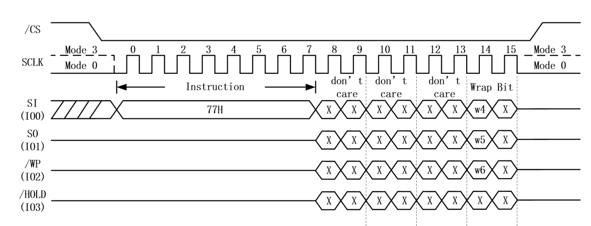
Figure 7.2.8. Set Burst with Wrap Instruction
