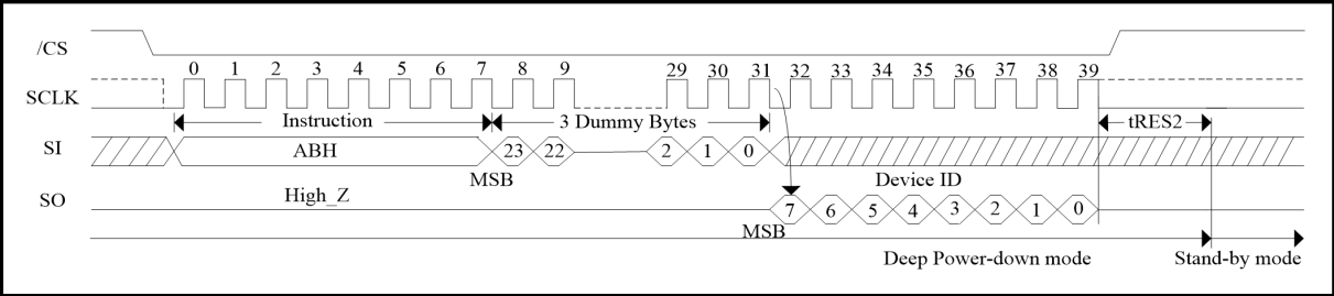
Figure 30. Release Power-Down/Read Device ID Sequence Diagram
