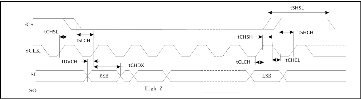
Figure 46. Output Timing
