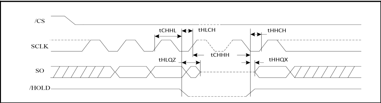
Figure 47. Hold Timing
