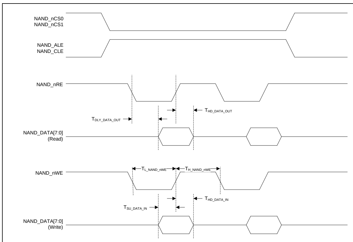
Figure 7.3-14 NAND Interface Timing Diagram
