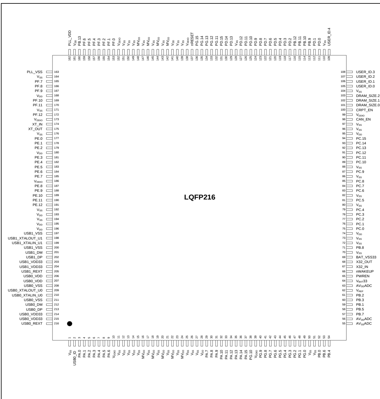
Figure 4.1-3 NUC980DFxxYC LQFP 216-pin Diagram
