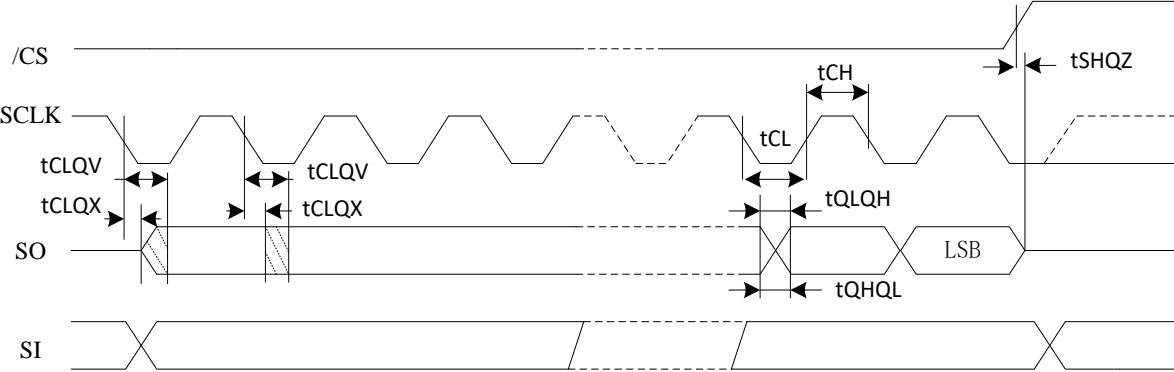
Figure 24. Output Timing
