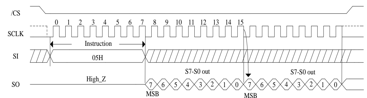
Figure 6. Read Status Register Sequence Diagram
