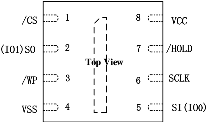
Figure 3. Pin Configuration DFN 2*3mm
