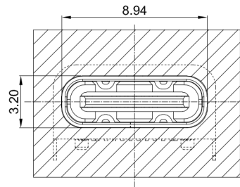
RECOMMENDED ASSEMBLY DRAWING
