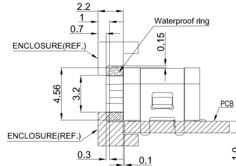
RECOMMENDED ASSEMBLY DRAWING
