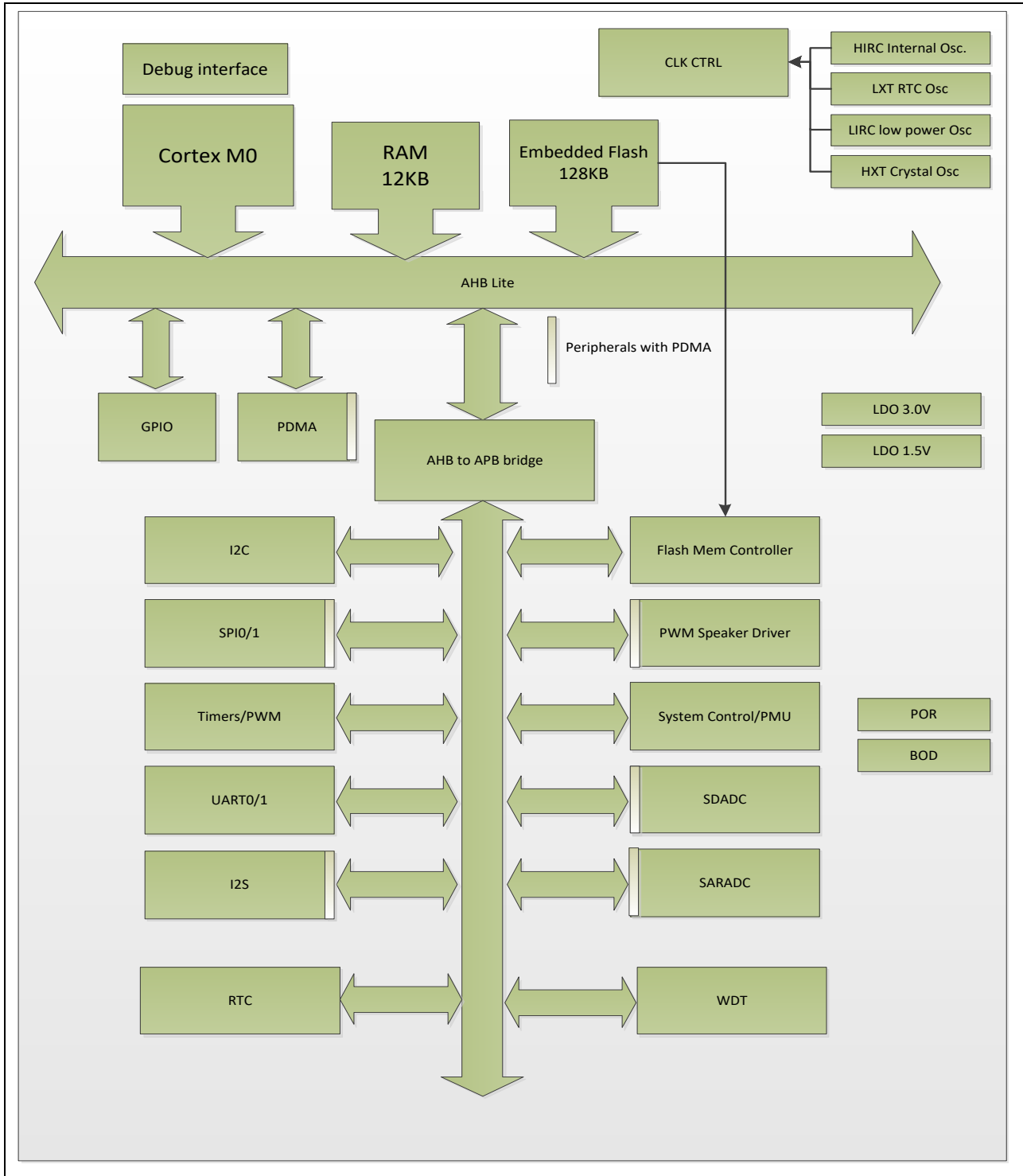
Figure 4-1 I91200 Block Diagram
