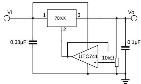
Fig.7 Adjustable output
