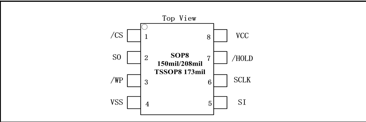
Figure 2. Pin Configuration SOP8 150mil/208 mil, TSSOP8 173mil
