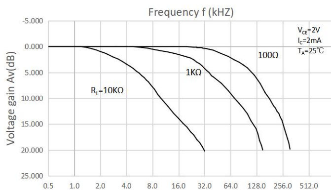
Fig.11 Frequency Response
