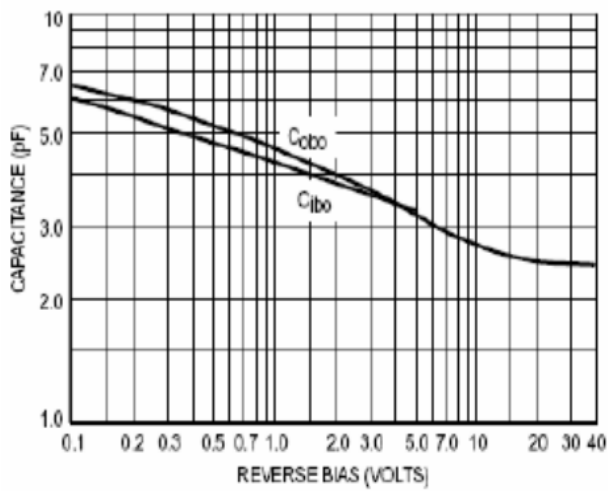
Figure 1 Capacitance
