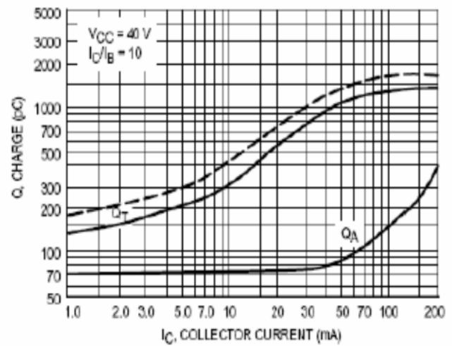
Figure 2 Charge Data
