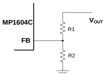
Figure 3: Feedback Network
