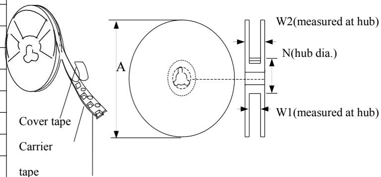
EIA Reel Dimensions
