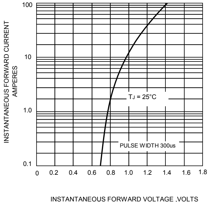
FIG.4-TYPICAL FORWARD CHARACTERISTICS
