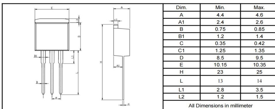
TO-262
