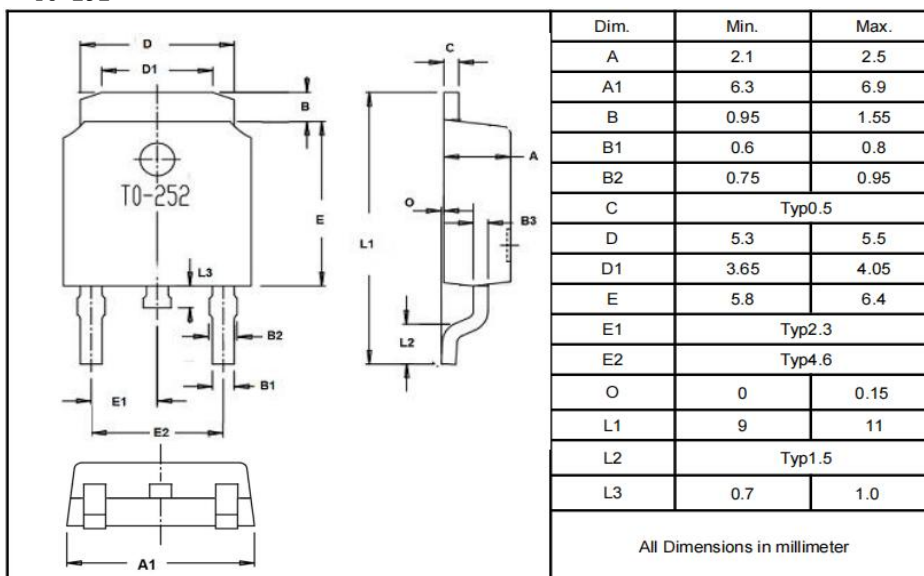
TO-252
