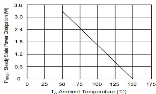
Figure 5. Steady State Power Dissipation Derating Curve
