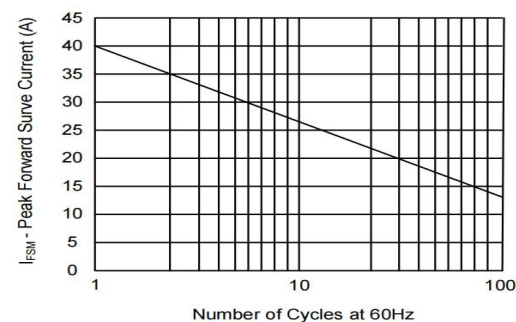
Figure 6. Maximum Non-Repetitive Forward Surge Current Uni-Directional Only
