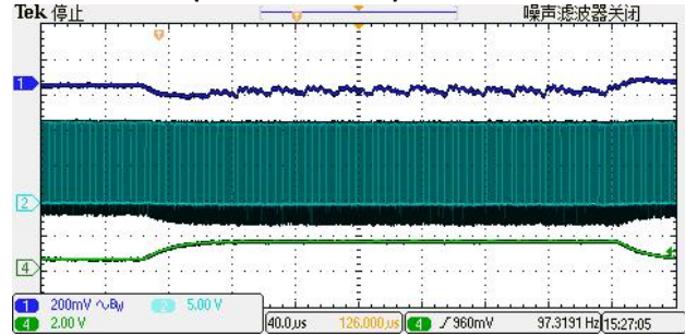
Load Transient(0.5A--1.5A Load)
