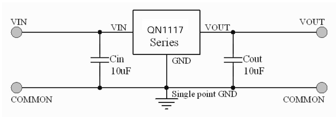
Application circuit of QN1117 fixed version
