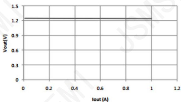
AMS1117S-ADJ Vout Vs. Iout
