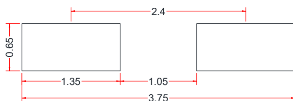
RECOMMENDED LAND PATTERN(Unit:mm)
