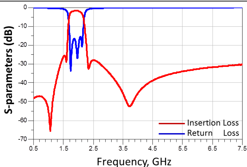
Typical Electrical Chart
