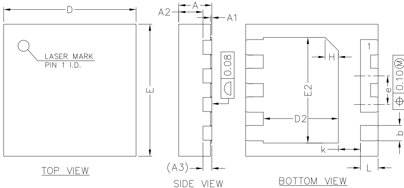
DFN3x3
