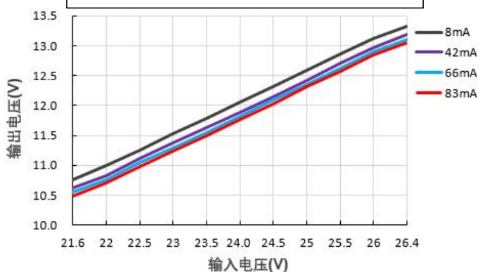
输出电压 Vs 输入电压@FN1-24S12BN
