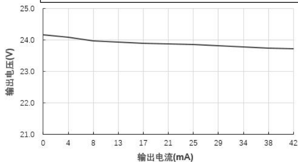
输出电压 Vs 输出电流 (Vin=24V)@FN1-24S24BN
