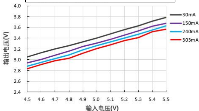
输出电压 Vs 输入电压@FN1-05S03BN
