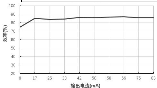
效率 Vs 输出电流 (Vin=5V)@FN1-05S12BN
