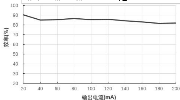
效率 Vs 输出电流 (Vin=3.3V)@FN1-03S05BN
