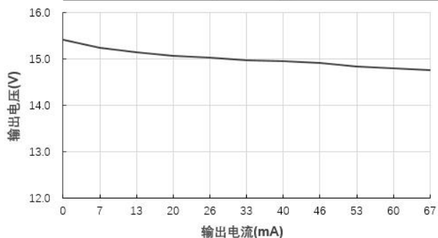
输出电压 Vs 输出电流 (Vin=12V)@FN1-12S15BN
