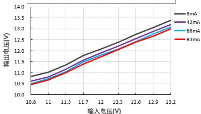
输出电压 Vs 输入电压@FN1-12S12BN
