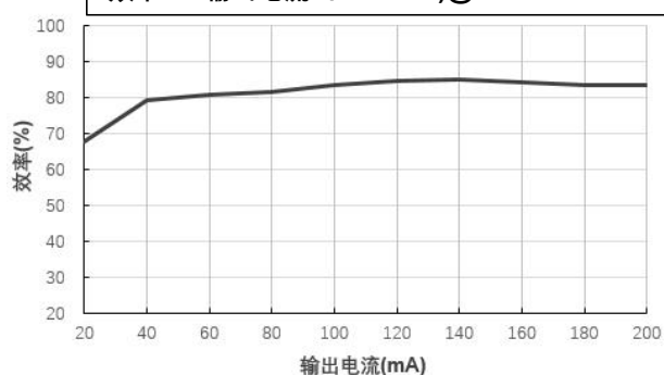
效率 Vs 输出电流 (Vin=12V)@FN1-12S05BN
