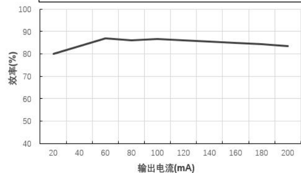
效率 Vs 输出电流 (Vin=5V)@FN1-05S05BN
