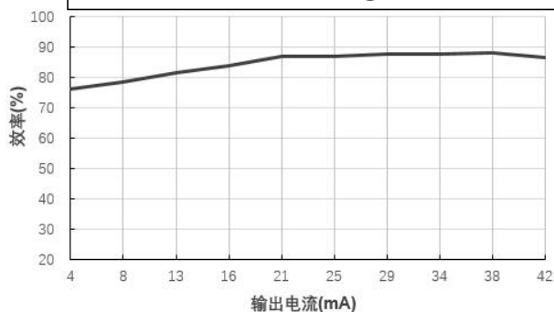
效率 Vs 输出电流 (Vin=5V)@FN1-05S24BN
