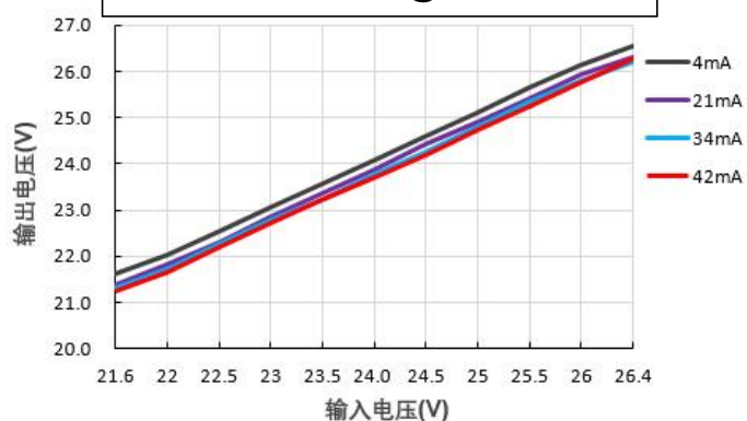
输出电压 Vs 输入电压@FN1-24S24BN
