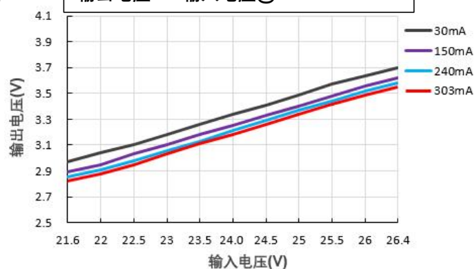
输出电压 Vs 输入电压@FN1-24S03BN
