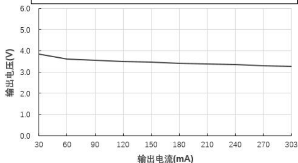
输出电压 Vs 输出电流 (Vin=3.3V)@FN1-03S03BN
