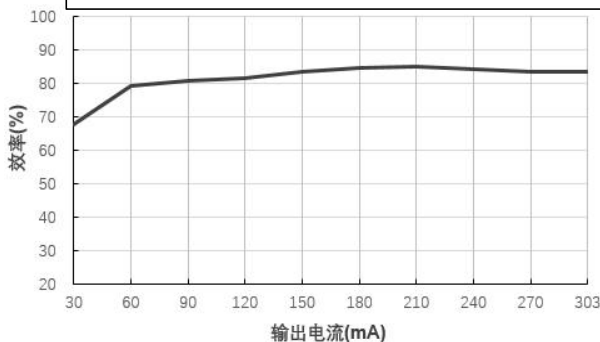
效率 Vs 输出电流 (Vin=12V)@FN1-12S03BN
