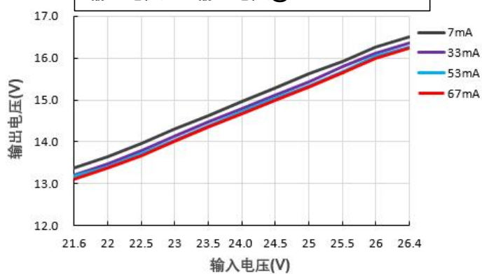
输出电压 Vs 输入电压@FN1-24S15BN
