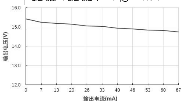
输出电压 Vs 输出电流 (Vin=5V)@FN1-05S15BN
