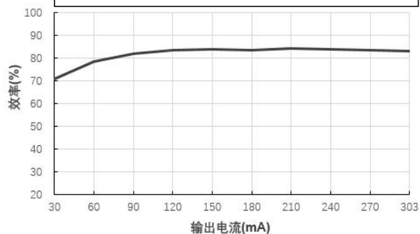
效率 Vs 输出电流 (Vin=5V)@FN1-05S03BN
