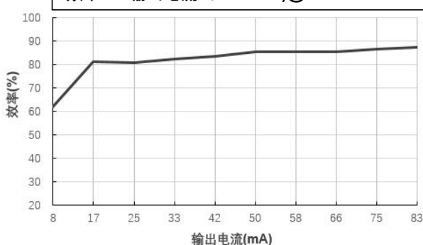
效率 Vs 输出电流 (Vin=12V)@FN1-12S12BN
