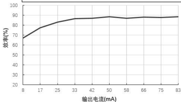
效率 Vs 输出电流 (Vin=24V)@FN1-24S12BN
