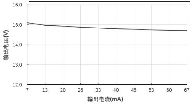
输出电压 Vs 输出电流 (Vin=24V)@FN1-24S15BN
