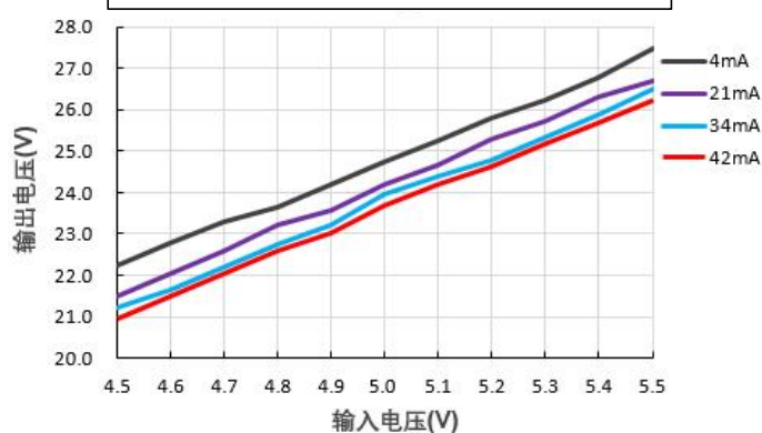
输出电压 Vs 输入电压@FN1-05S24BN
