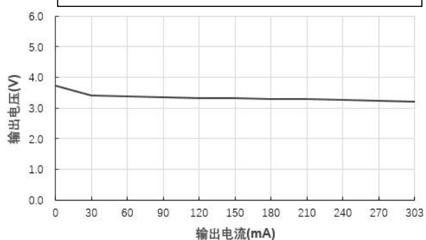
输出电压 Vs 输出电流 (Vin=12V)@FN1-12S03BN
