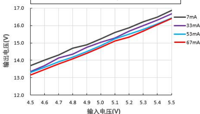
输出电压 Vs 输入电压@FN1-05S15BN
