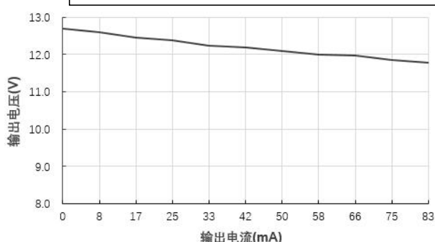
输出电压 Vs 输出电流 (Vin=5V)@FN1-05S12BN
