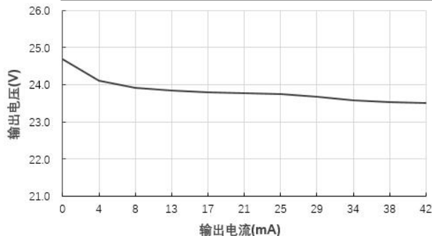
输出电压 Vs 输出电流 (Vin=12V)@FN1-12S24BN
