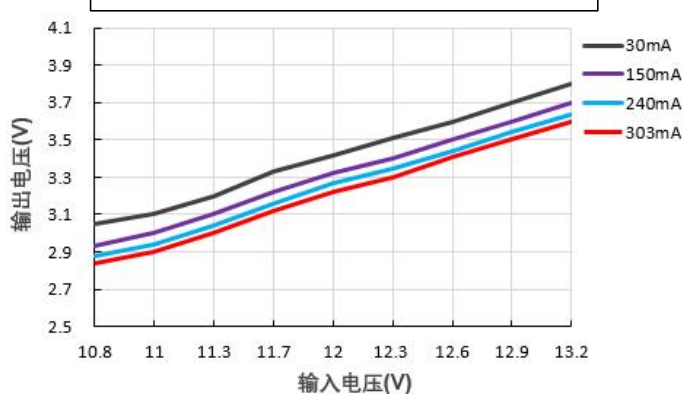
输出电压 Vs 输入电压@FN1-12S03BN
