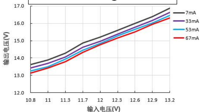
输出电压 Vs 输入电压@FN1-12S15BN
