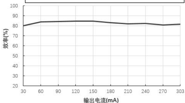
效率 Vs 输出电流 (Vin=3.3V)@FN1-03S03BN
