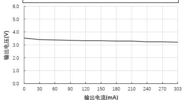
输出电压 Vs 输出电流 (Vin=5V)@FN1-05S03BN
