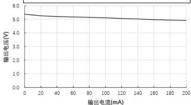
输出电压 Vs 输出电流 (Vin=12V)@FN1-12S05BN
