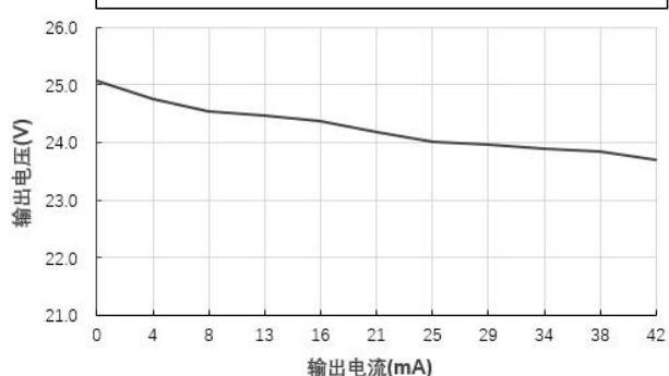
输出电压 Vs 输出电流 (Vin=5V)@FN1-05S24BN
