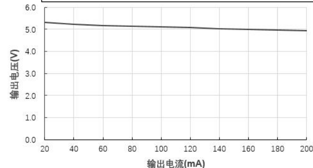
输出电压 Vs 输出电流 (Vin=24V)@FN1-24S05BN
