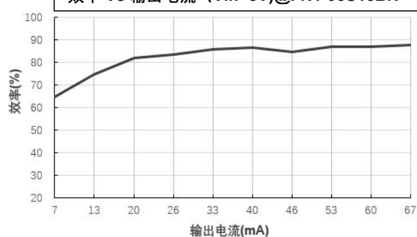
效率 Vs 输出电流 (Vin=5V)@FN1-05S15BN
