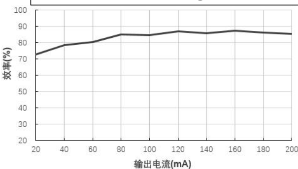
效率 Vs 输出电流 (Vin=24V)@FN1-24S05BN
