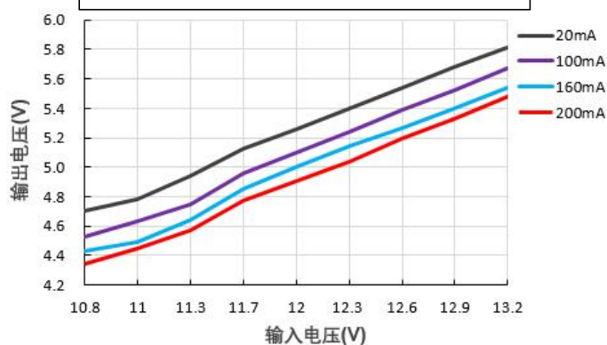
输出电压 Vs 输入电压@FN1-12S05BN
