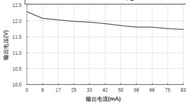
输出电压 Vs 输出电流 (Vin=12V)@FN1-12S12BN
