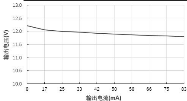
输出电压 Vs 输出电流 (Vin=24V)@FN1-24S12BN
