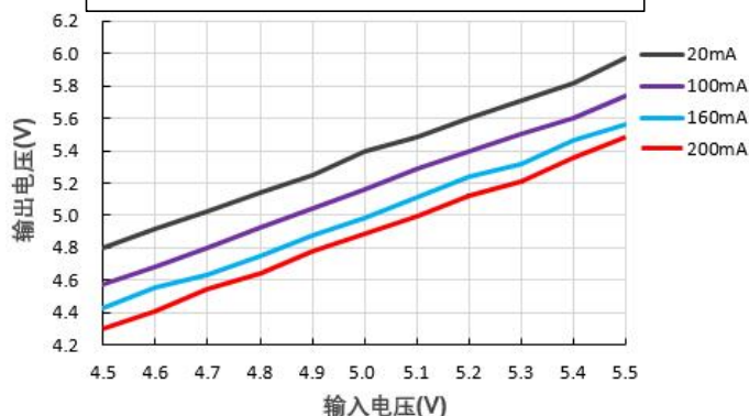
输出电压 Vs 输入电压@FN1-05S05BN
