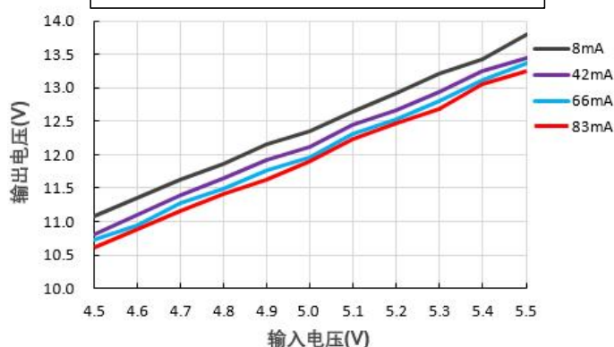
输出电压 Vs 输入电压@FN1-05S12BN
