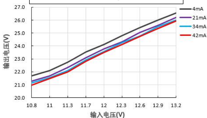
输出电压 Vs 输入电压@FN1-12S24BN
