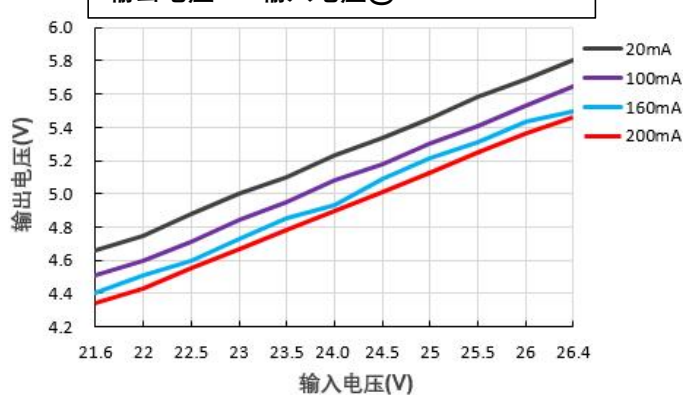
输出电压 Vs 输入电压@FN1-24S05BN
