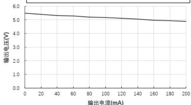
输出电压 Vs 输出电流 (Vin=5V)@FN1-05S05BN
