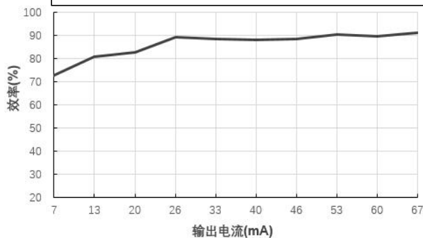
效率 Vs 输出电流 (Vin=24V)@FN1-24S15BN
