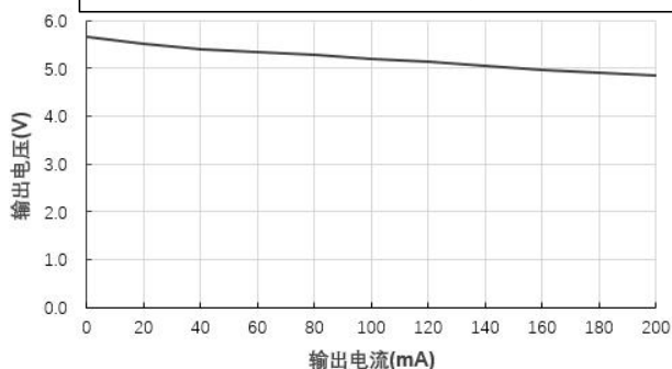
输出电压 Vs 输出电流 (Vin=3.3V)@FN1-03S05BN
