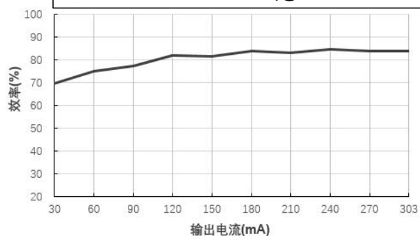
效率 Vs 输出电流 (Vin=24V)@FN1-24S03BN
