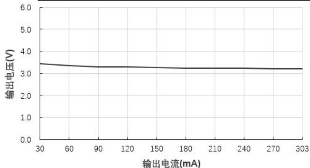
输出电压 Vs 输出电流 (Vin=24V)@FN1-24S03BN
