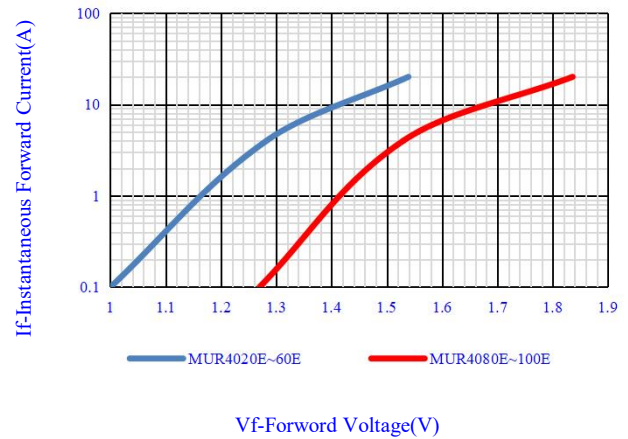
Fig.2-Typical Instantaneous Forward
