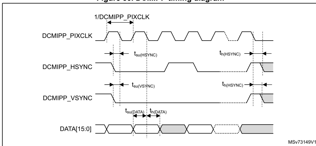
Figure 50. DCMIPP timing diagram
