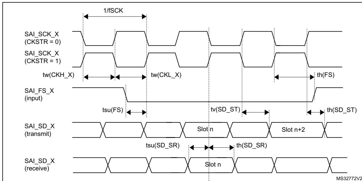
Figure 61. SAI target timing waveforms
