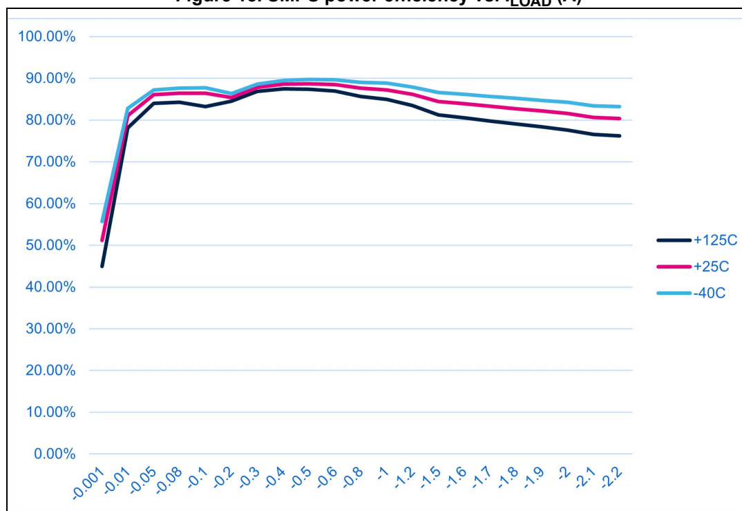
Figure 18. SMPS power efficiency vs. I_{LOAD} (A)
