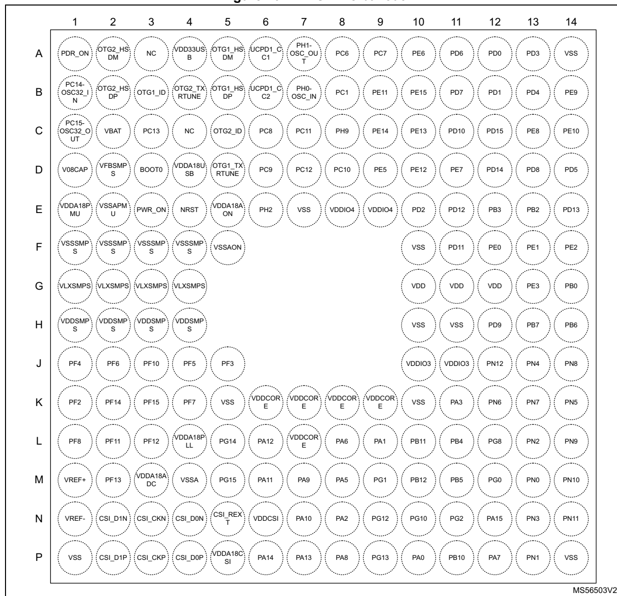
Figure 10. VFBGA178 ballout
