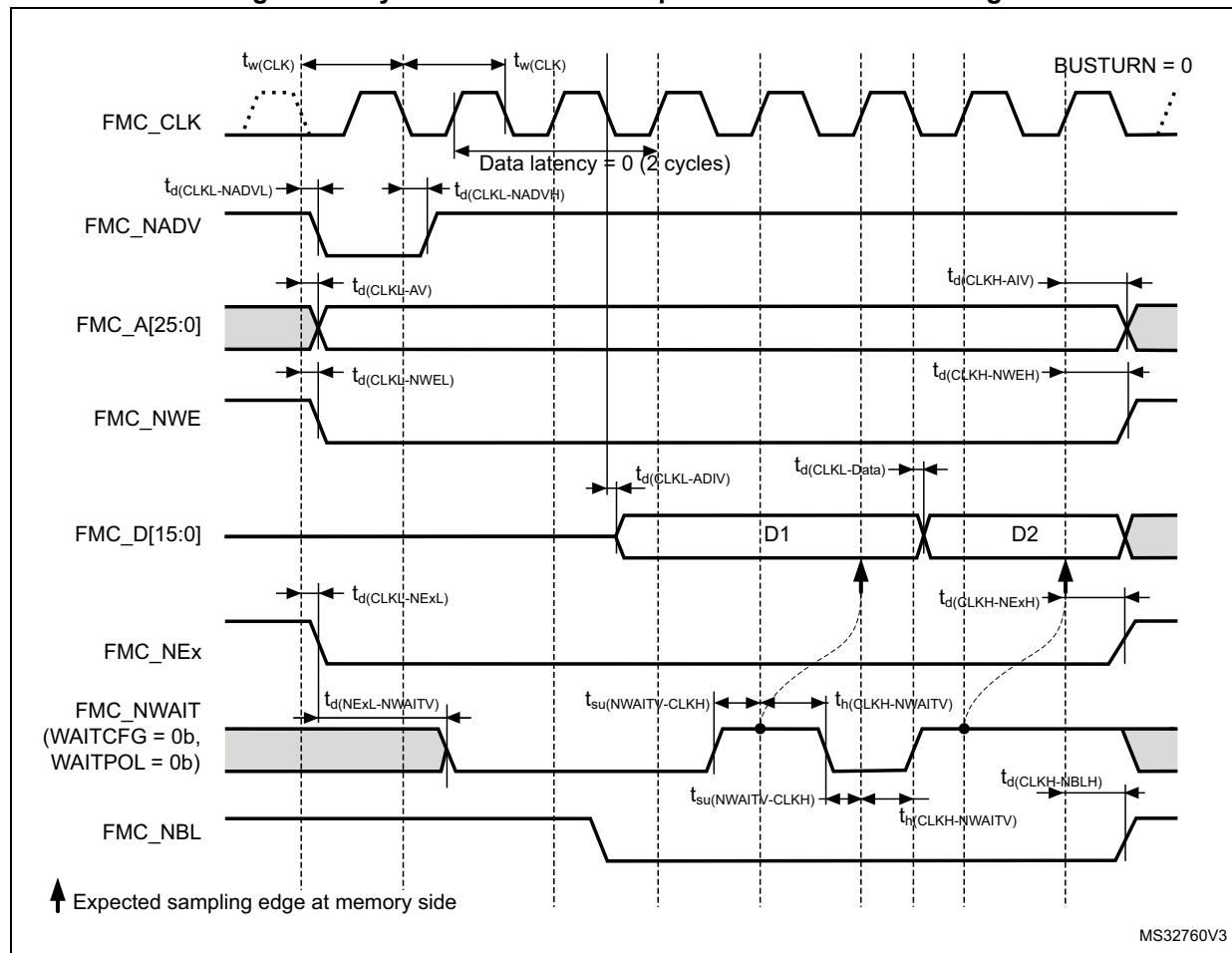
Figure 31. Synchronous non multiplexed PSRAM write timings
