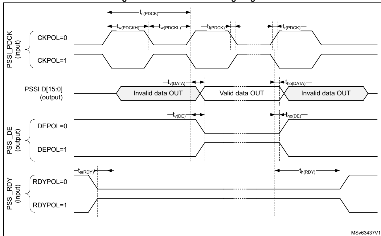
Figure 51. PSSI transmit timing diagram
