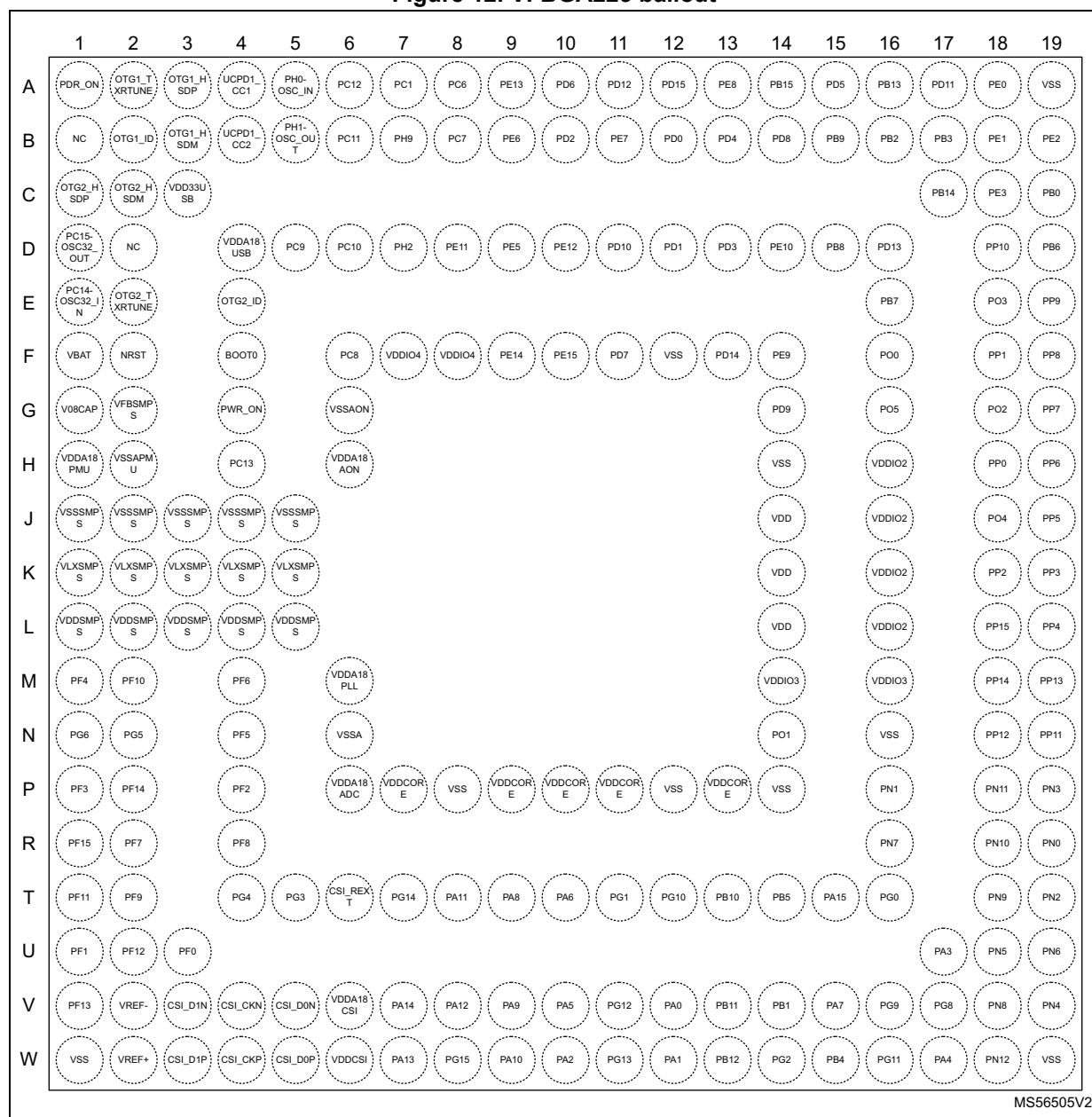
Figure 12. VFBGA223 ballout
