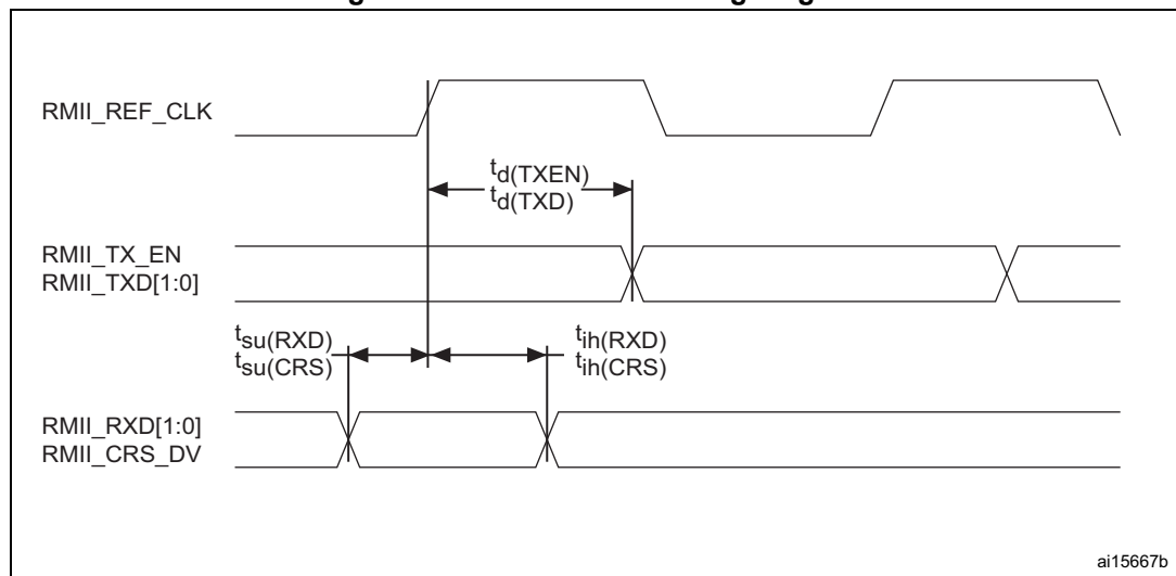
Figure 63. Ethernet RMII timing diagram
