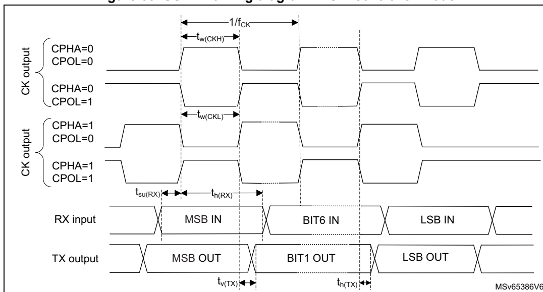
Figure 65. USART timing diagram in SPI controller mode
