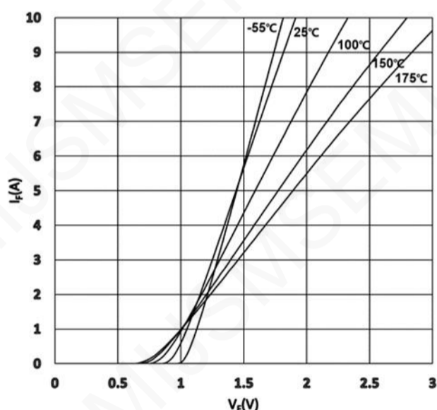
Figure 1: Forward Characteristics
