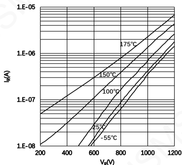
Figure 2: Reverse Characteristics
