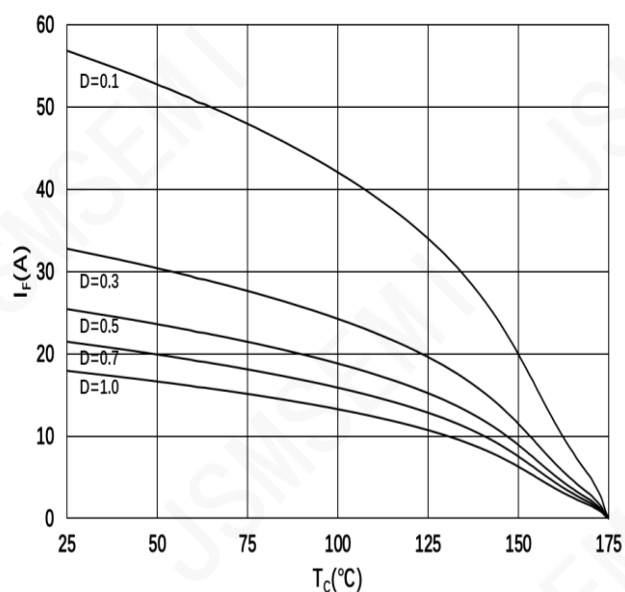
Figure 3: Current Derating
