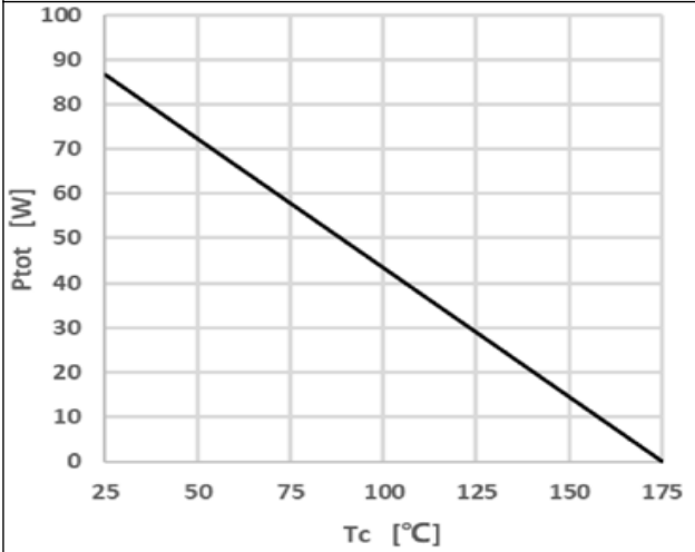
Figure 6. Power Derating
