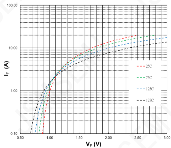
Figure 2. Forward Characteristics
