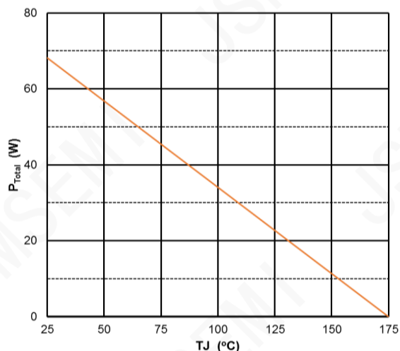
Figure 4. Power Derating
