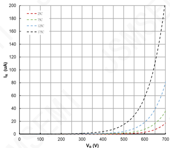
Figure 3. Reverse Characteristics
