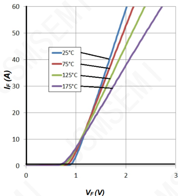
Figure 1. Forward Characteristics
