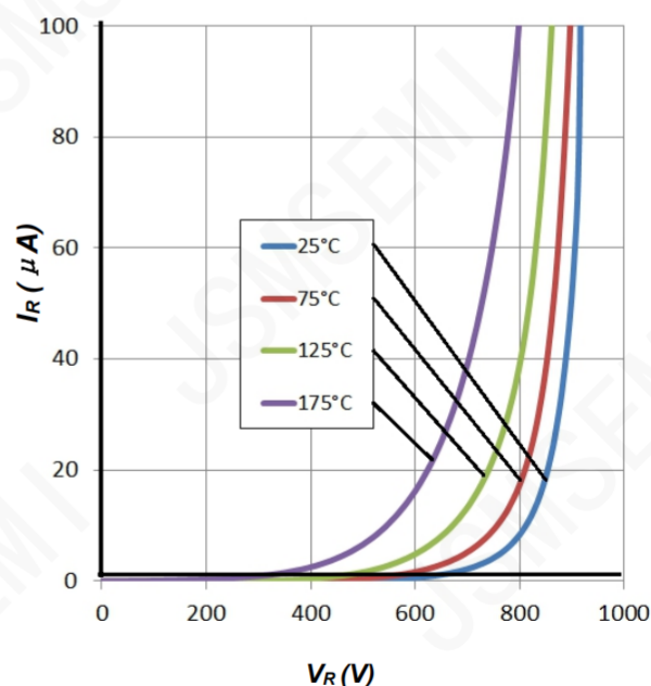
Figure 2. Reverse Characteristics
