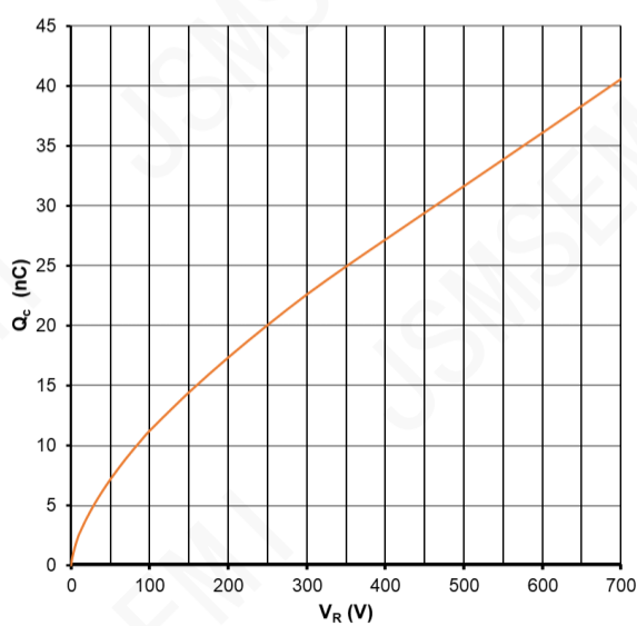
Figure 6. Recovery Charge vs Reverse Voltage
