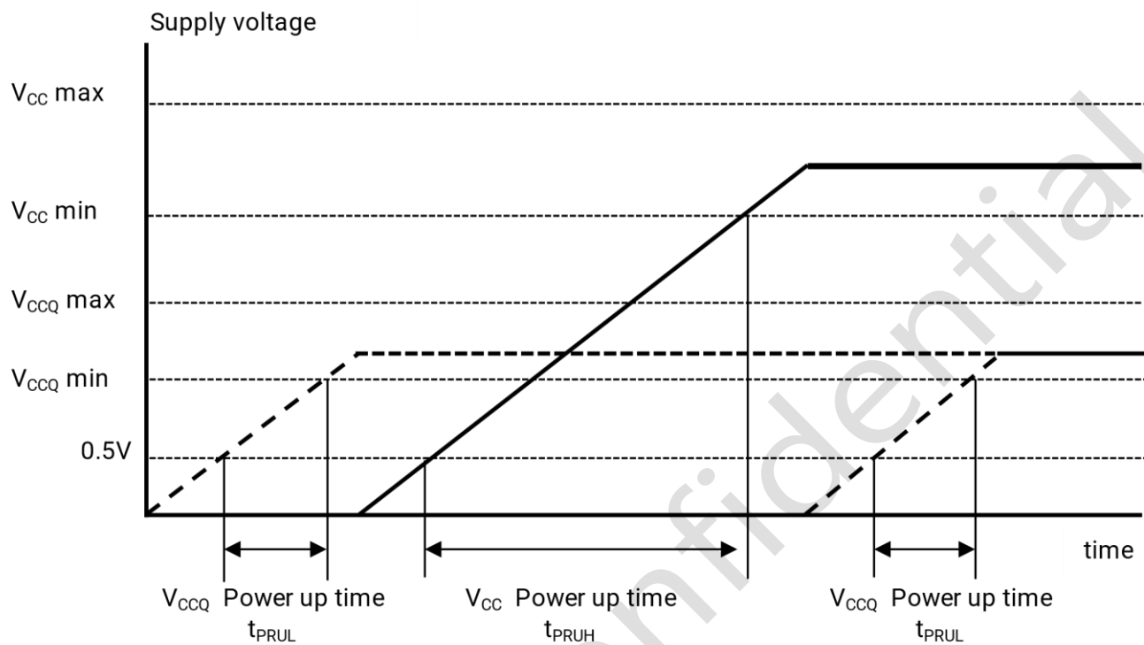
Figure 15 Power-on Sequence
