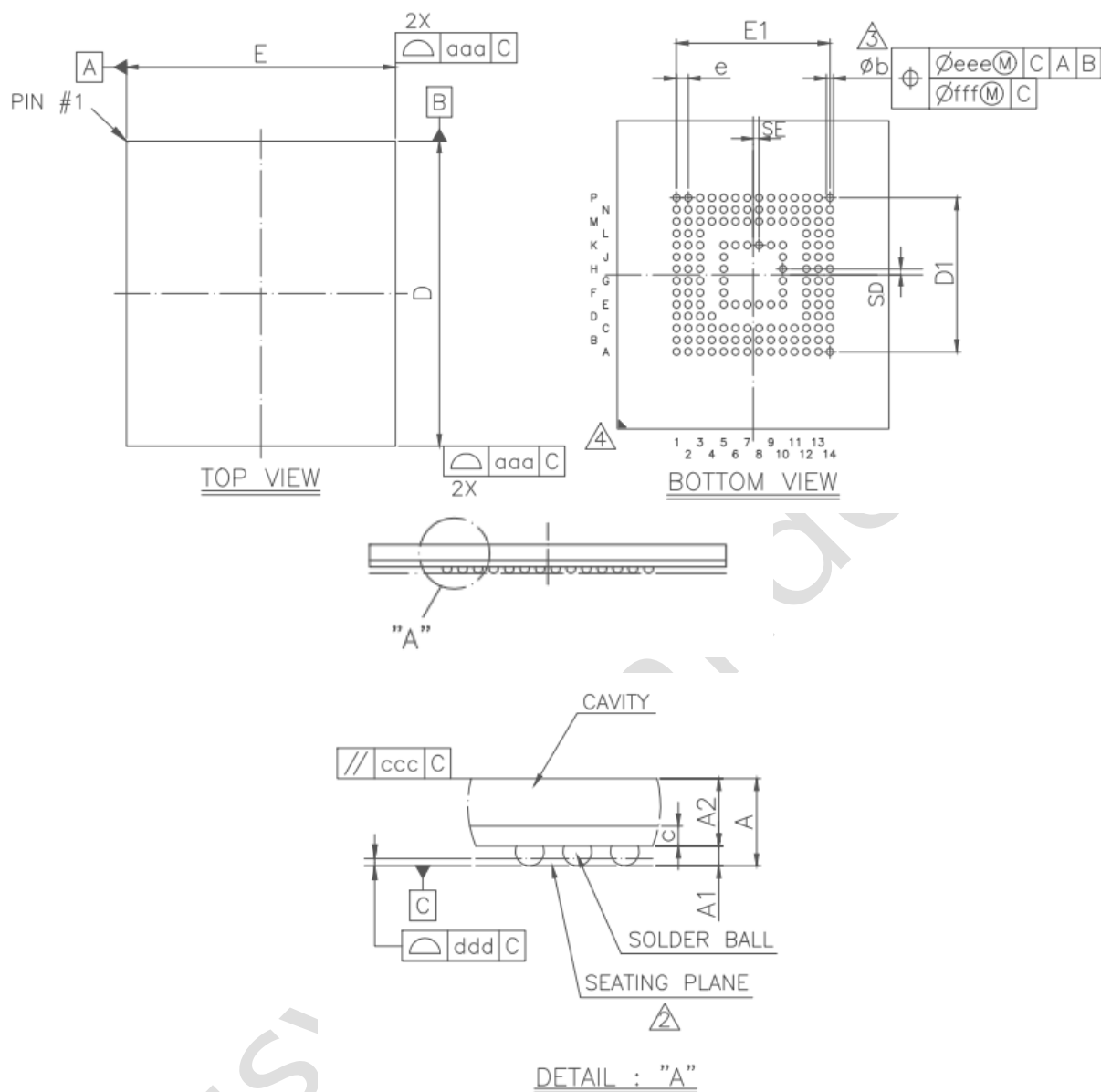
Figure 3 Package Dimension
