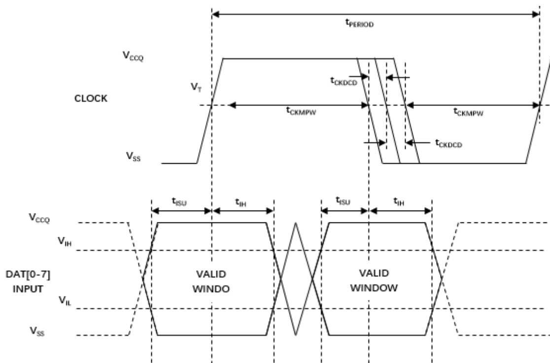
Figure 11 HS400 Device Input Timing
