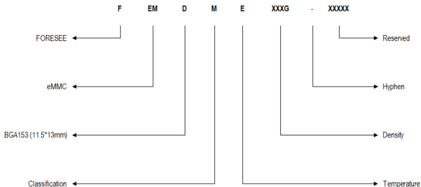
Figure 1 Part Number Decoder
