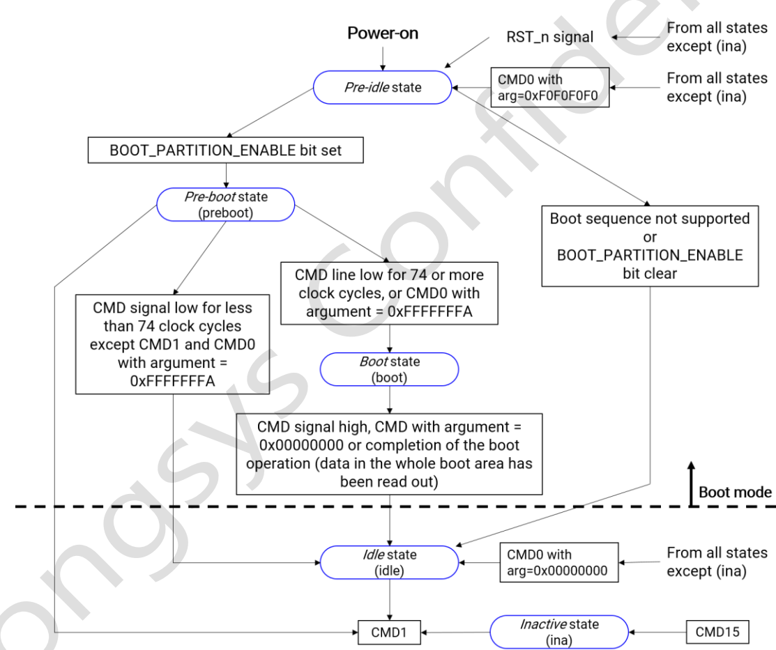
Figure 8 State Diagram (Boot Mode)
