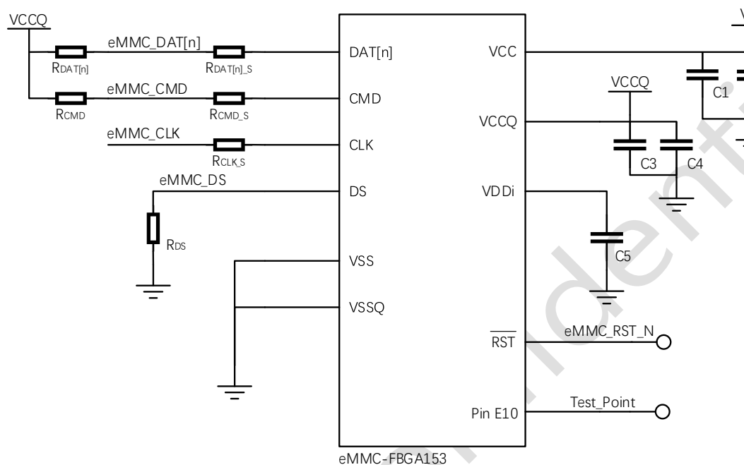
Figure 9 eMMC Reference Schematics
