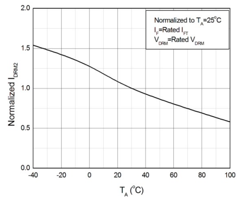
Fig.12 Normalized Leakage in Inhibit State Ambient Temperature
