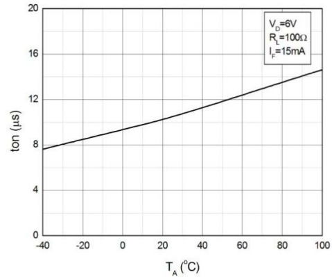
Fig.14 Turn On Time vs. Ambient Temperature
