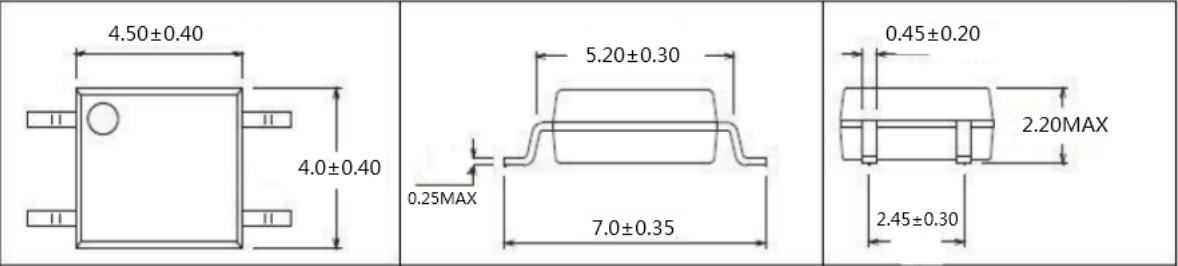
4-pin SOP
