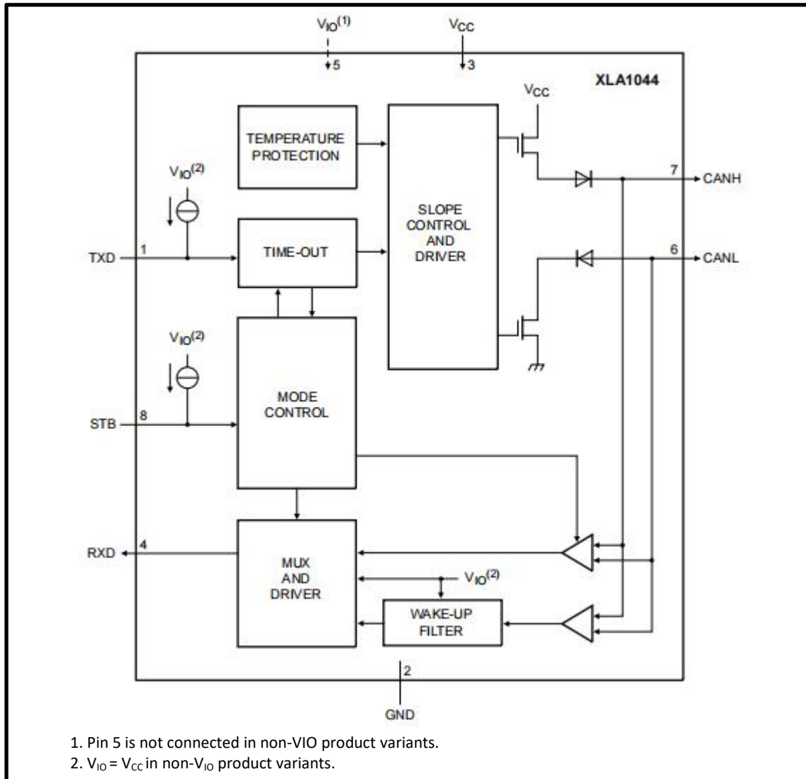
Figure 1. Block diagram
