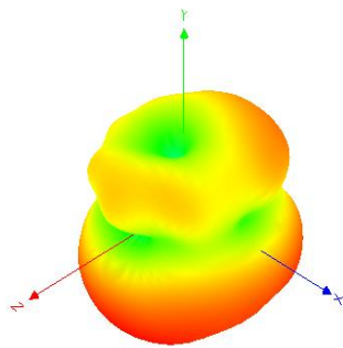
Frequency (MHz) : 2400
