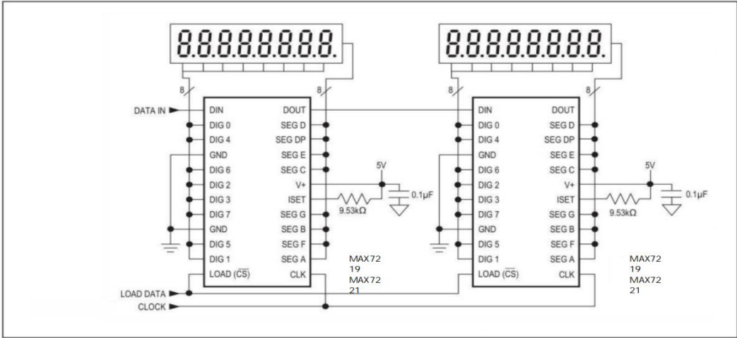
Figure 3. Cascading MAX7219 / MAX7221 to Drive 16 Seven-Segment LED Digits
