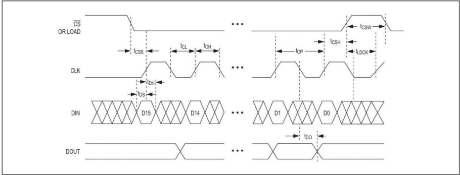
Figure 1. Timing Diagram
