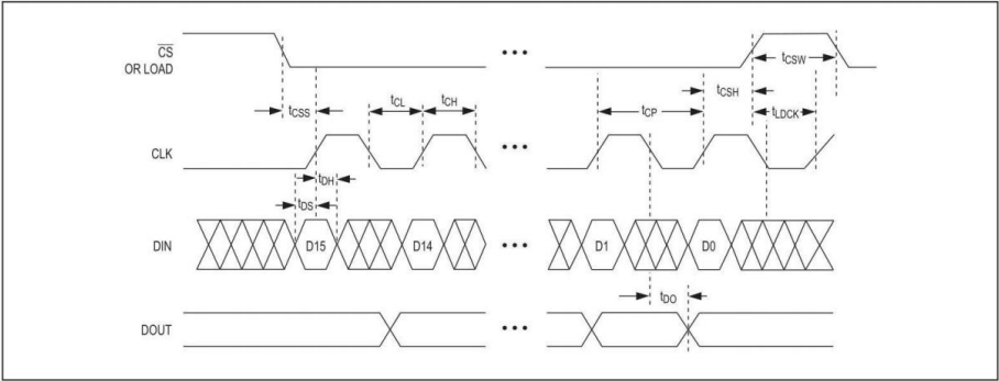
Figure 1. Timing Diagram
