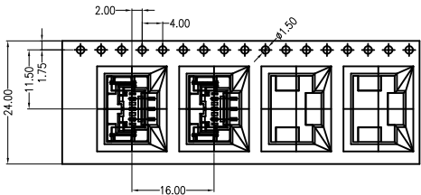
02~03 CONTACTS
