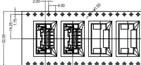
04~10 CONTACTS
