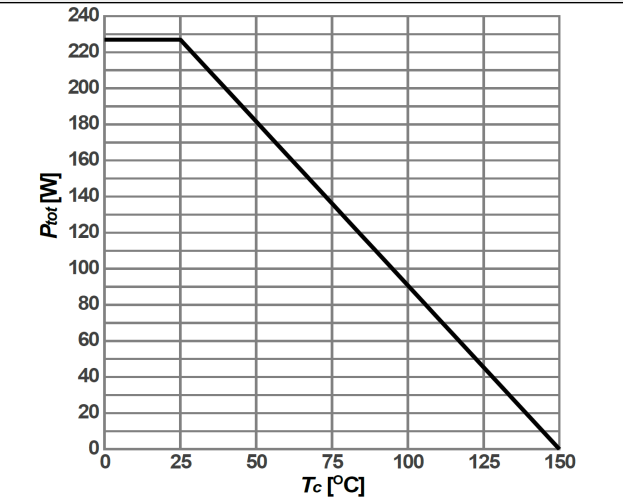
Figure 4: Power dissipation For TO-220、TO-247、TO-263
