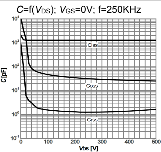
Figure 16: Typ. capacitances
