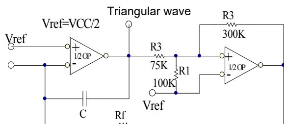
Function Generator
