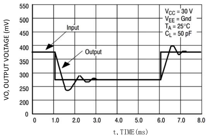
Small Signal Voltage Follower Pulse Response
