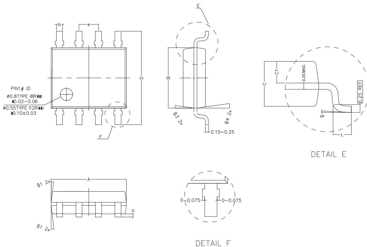
COMMON DIMENSIONS (UNITS OF MEASURE IS mm)
