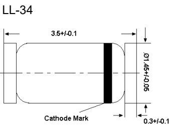
Glass case MiniMELF Dimensions in mm
