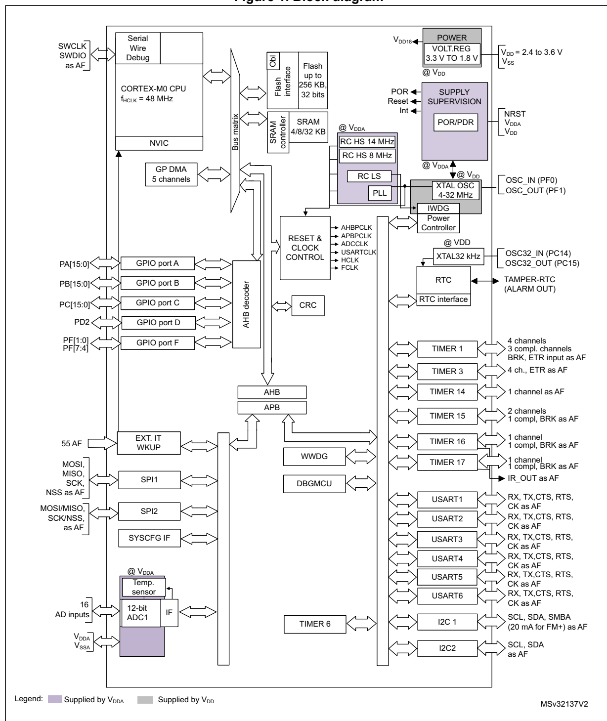
Figure 1. Block diagram
