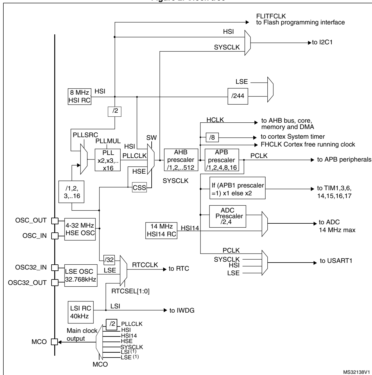
Figure 2. Clock tree
