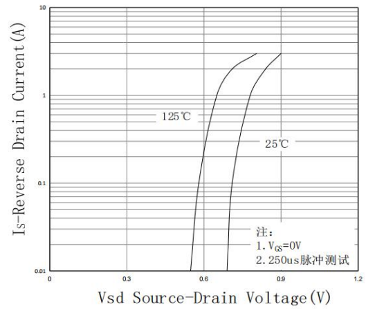
Fig.8 Body Diode Characteristic
