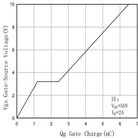
Fig.7 Gate-Charge Characteristic
