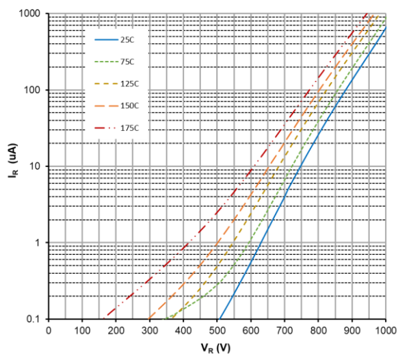
Figure 3. Reverse Characteristics
