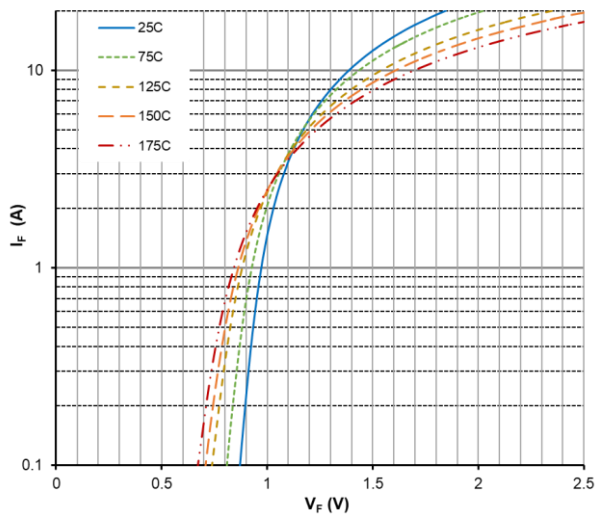
Figure 2. Forward Characteristics
