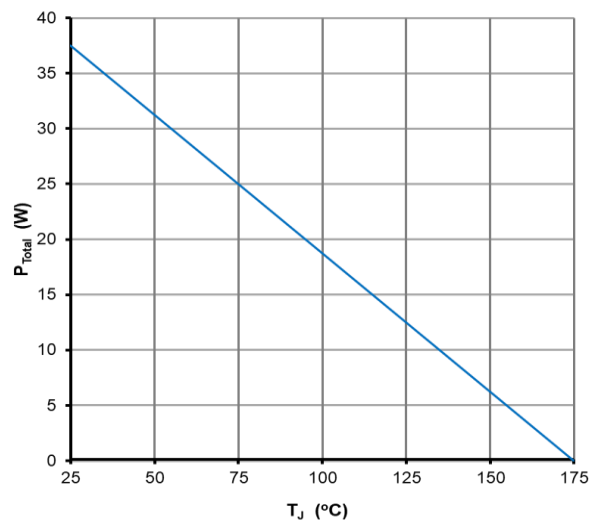
Figure 4. Power Derating
