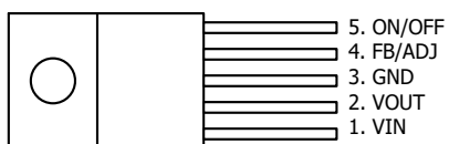
TO-220-5L
