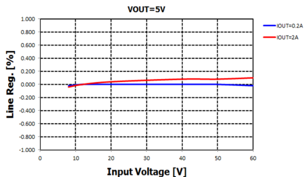
Line Regulation vs. VIN
