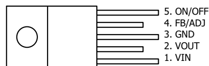
TO-220TV-5L
