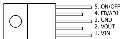
TO-220TV-5L
