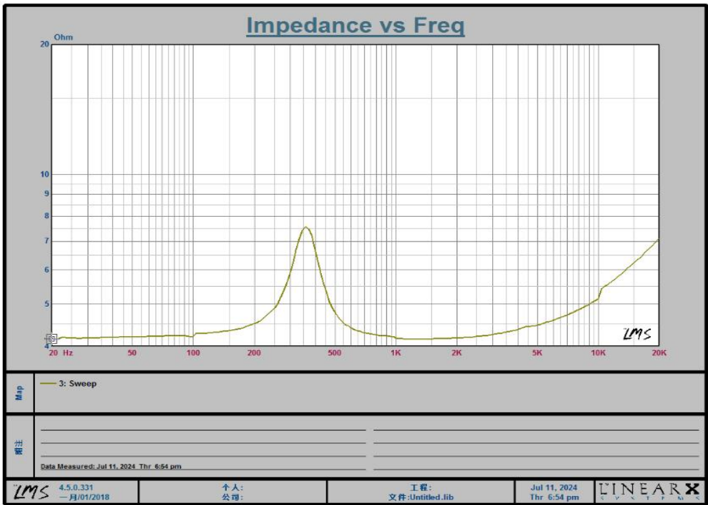
产品阻抗曲线图 Product impedance curve
