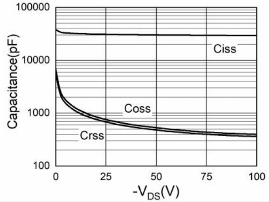
Figure 8. Capacitance
