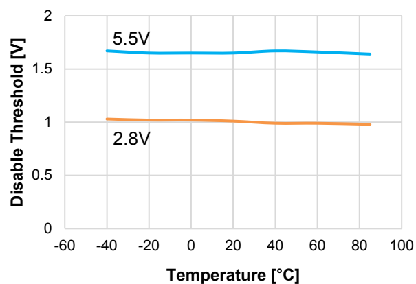
Disable Threshold vs. Temperature
