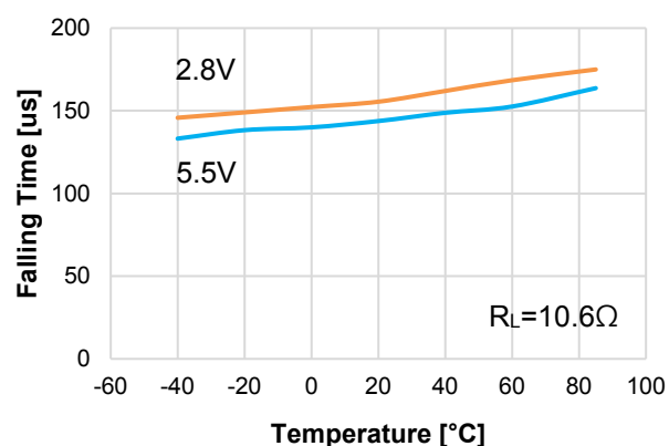
Falling Time vs. Temperature
