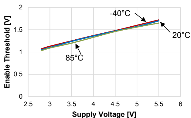
Enable Threshold vs. Supply Voltage
