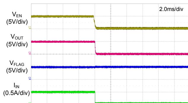
Turn OFF
