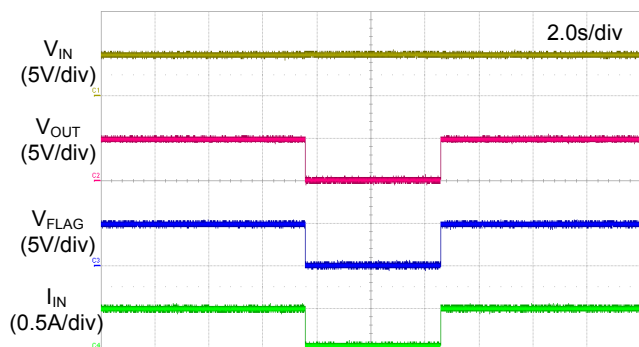
Thermal Shutdown
