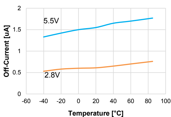
Off-Current vs. Temperature
