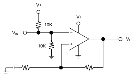
NON-INVERTING AMPLIFIER
