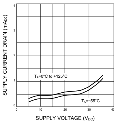
SUPPLY CURRENT
