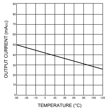
CURRENT LIMITING
